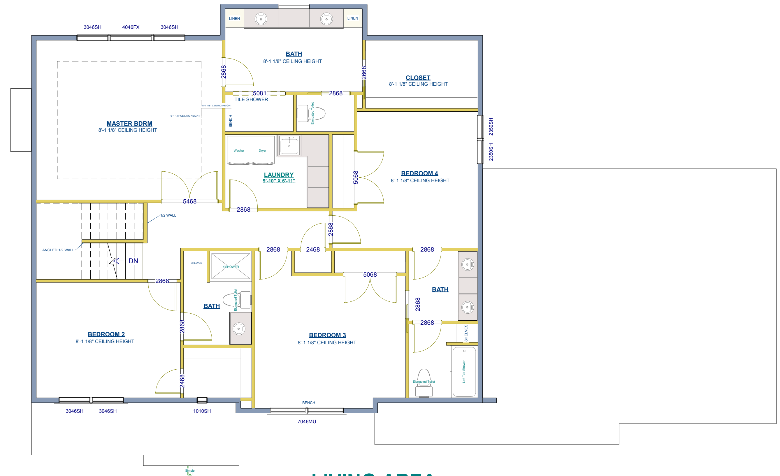
LIVING AREA 1483 SQ.FT
